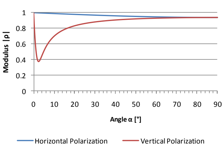
Fig. 10 : Sea water reflection coeff. modulus
