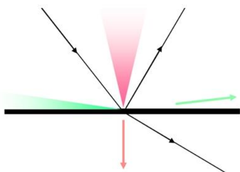
Fig. 8 : Steep angles transmit the most, while shallow (grazing) angles reflect
