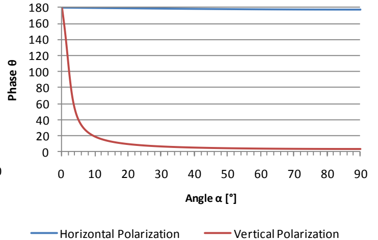
Fig. 11 : Sea water reflection coeff. phase
