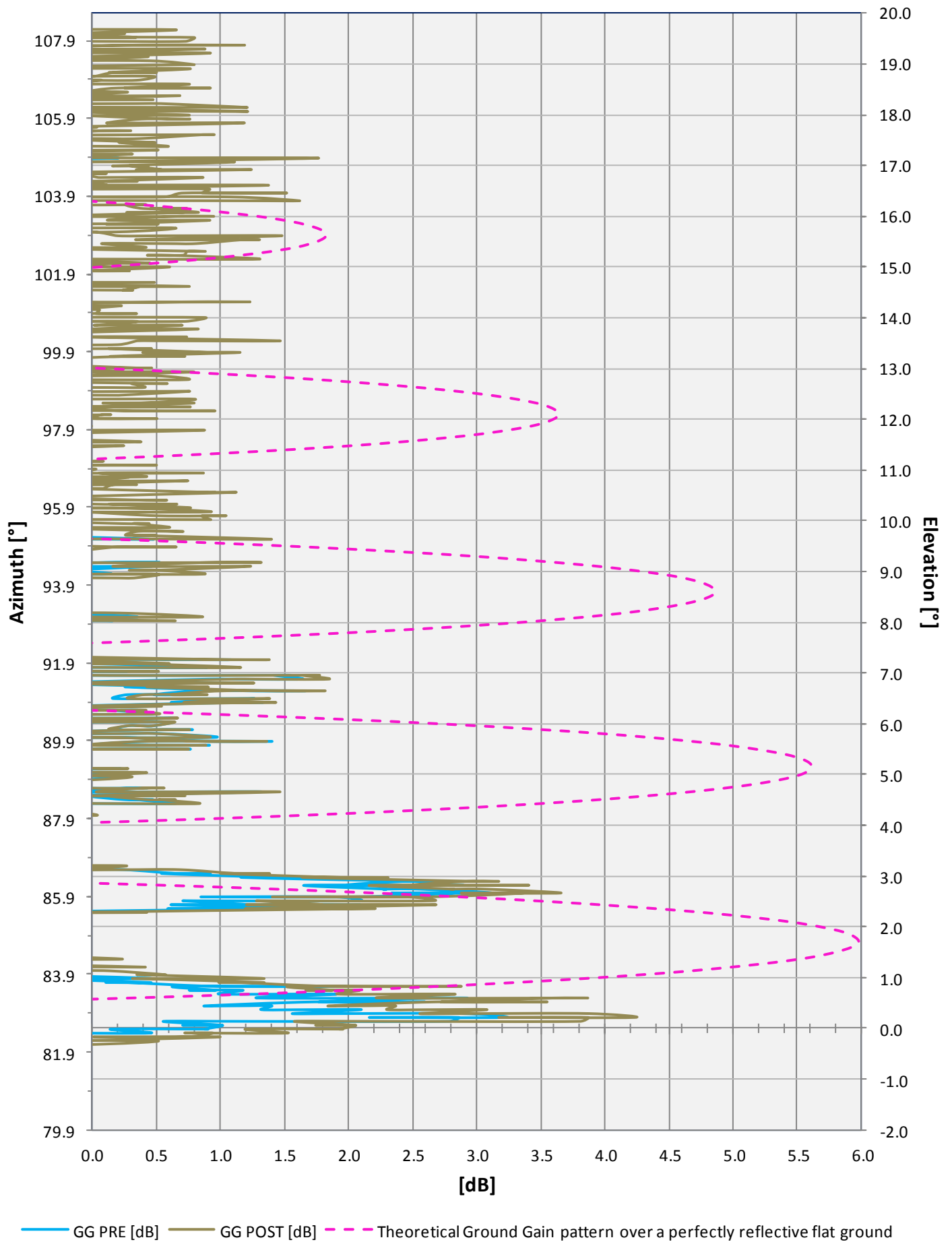
Fig. 28 : Ground Gain at sun rise
